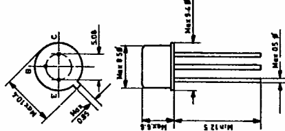
TO-39
